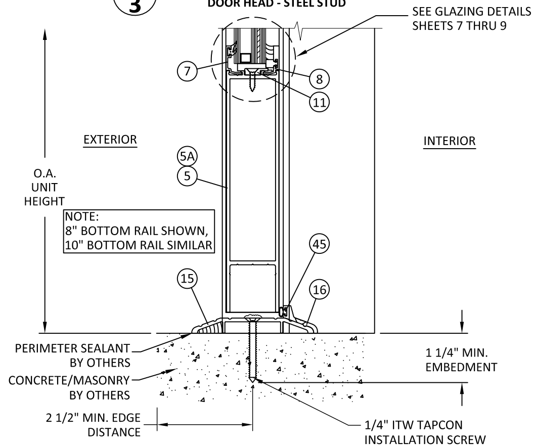
D 3 VERTICAL SECTION BOTTOM RAIL - CONCRETE/MASONRY
