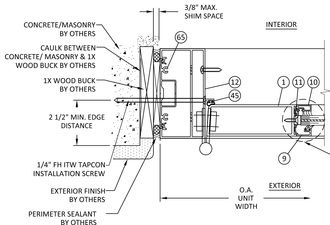
E 4 HORIZONTAL SECTION DOOR JAMB - CONCRETE/MASONRY STANDARD BUTT HINGE
