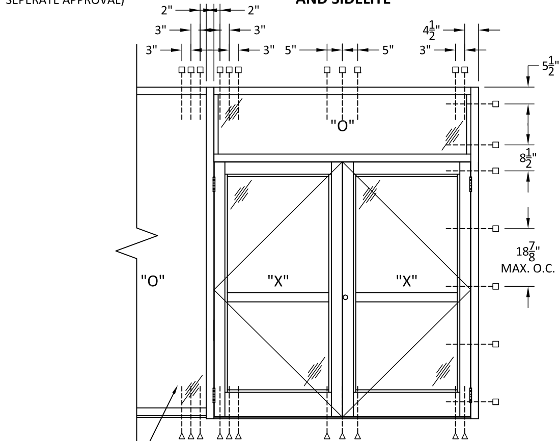
ANCHOR LAYOUT B DOUBLE DOOR WITH TRANSOM AND SIDELITE
