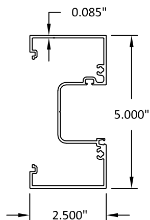
58 HEAD/JAMB/MULLION (INS)
