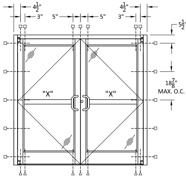
ANCHOR LAYOUT A DOUBLE DOOR
