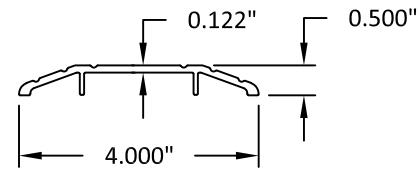
15 4" THRESHOLD
