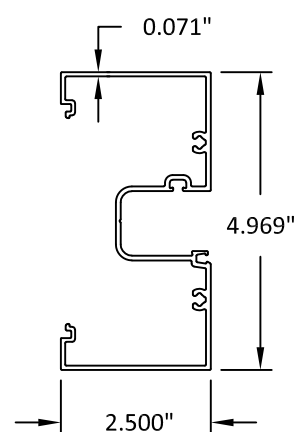
51 HEAD/JAMB/MULLION (MONO)
