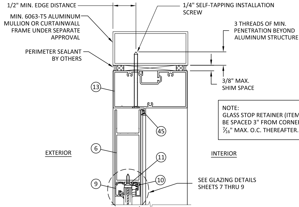
A 3 VERTICAL SECTION DOOR HEAD - ALUMINUM MULLION
