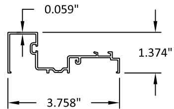
18 TRANSOM ADAPTOR (INS)
